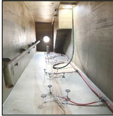
FRACAIR Magnetic Aeration Wastewater and Water Treatment System
